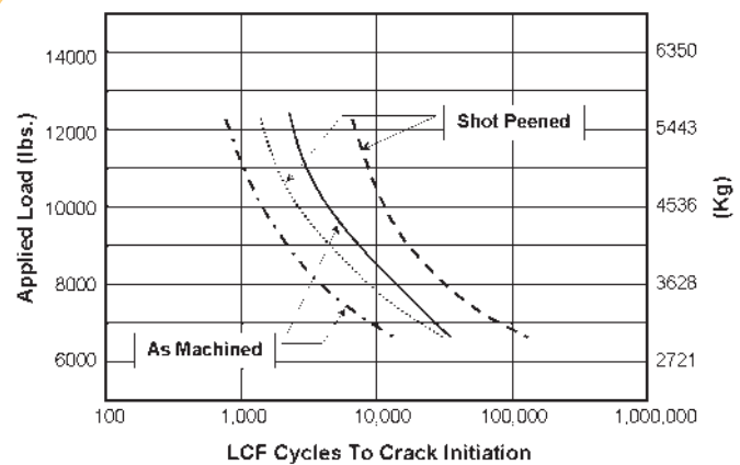
FIGURE 2-5 LCF Benefits from Shot Peening Notched Ti8-1-1
