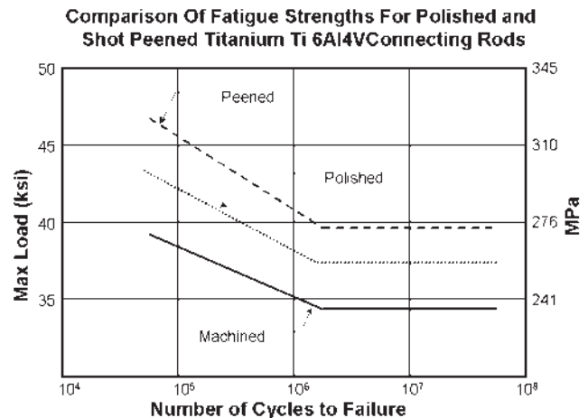
FIGURE 2-4 Comparison of Fatigue Strengths for Polished and Shot Peened Titanium Ti6Al4V
