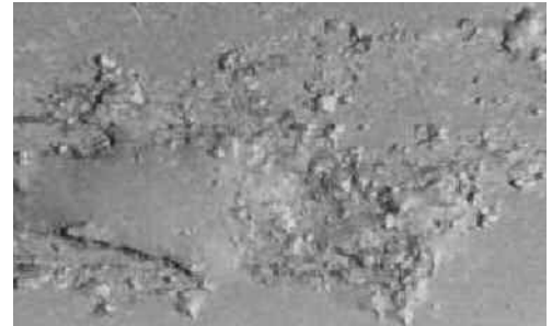
FIGURE 10-8 Exfoliation Corrosion
